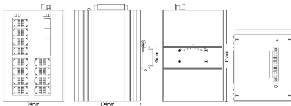
Front view
